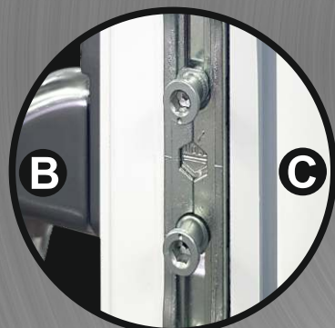
Opposing Twin Steel Locking Cams & Key Locking Handle
